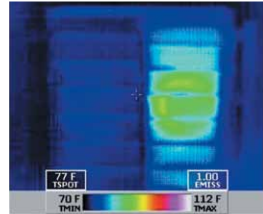
Thermal energy tests demonstrate the insulating value of Haven.
